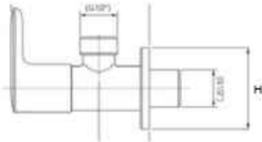
Angle Valve Height H mm
