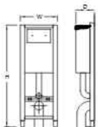
Toilets In-Wall Tank (W,D,H mm)
