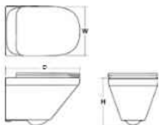
Commercial Bowel Toilet (W,D,H mm)
