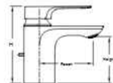
Sensor Faucet / Kitchen Faucet (Reach R, Total Height H mm, Reach, Height of Aerator mm)
