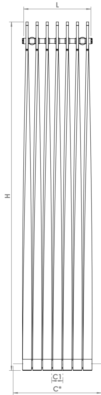
Front View
